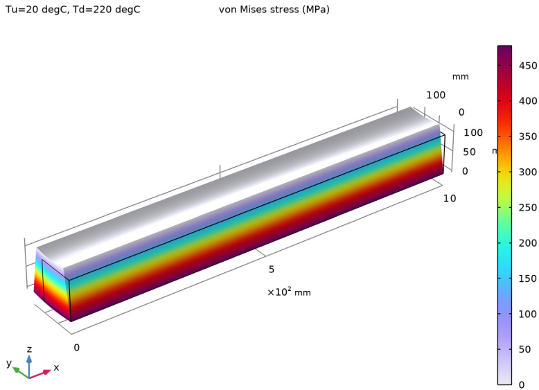
Figure 2: Stress distribution for T_u = 20^\circ\text{C} and T_d = 220^\circ\text{C} .
