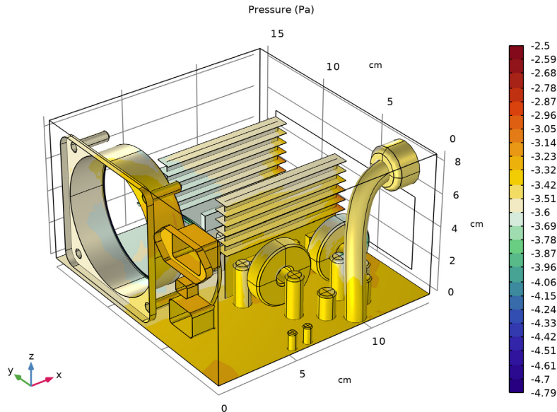
Figure 3: Pressure isosurfaces show the head loss created by electronic components.
