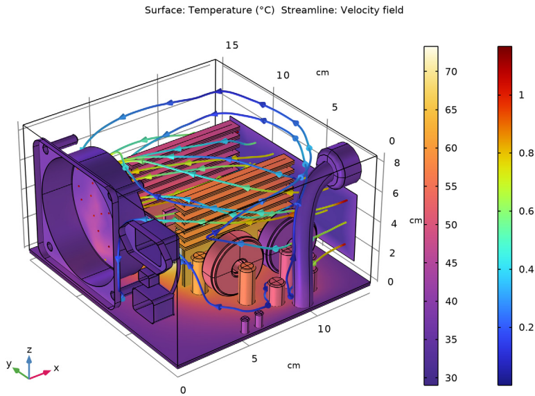
Figure 2: Temperature and fluid velocity fields.
