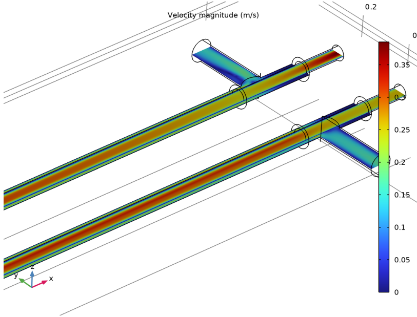
Figure 3: Velocity magnitude inside the pipes, zoomed at inlet and outlet regions.
