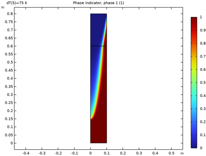
Figure 2: The fraction of solid phase for \Delta T = 75 K shows a gradual transition between the liquid and solid phase.
