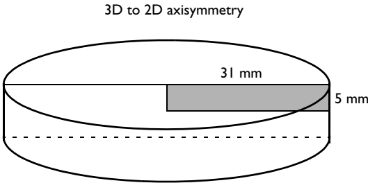
Figure 2: Geometry of the chicken patty.
