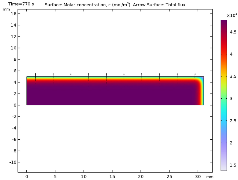
Figure 6: Moisture concentration after 770 s at a cooking temperature of 135°C.
