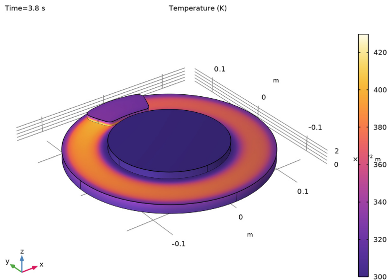
Figure 4: Surface temperature of the brake disc and pad just before releasing the brake ( t = 3.8 s).
