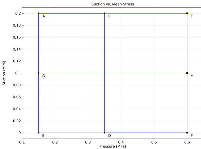
Figure 3: Load paths.
