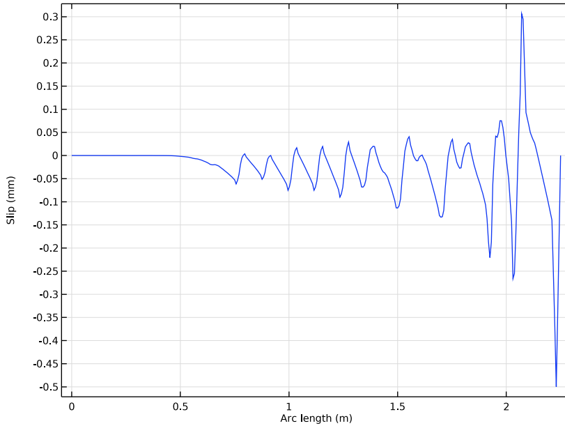
Figure 7: Slip between concrete and the rebar at the last step of the analysis.
