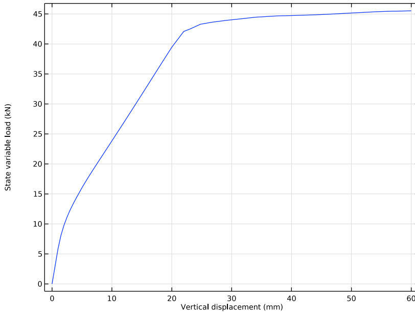
Figure 3: Load versus displacement curve of the reinforced concrete beam.
