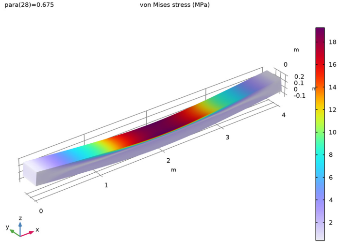
Figure 10: von Mises stress in the reinforced beam after adding the Ottosen criterion for the concrete.
