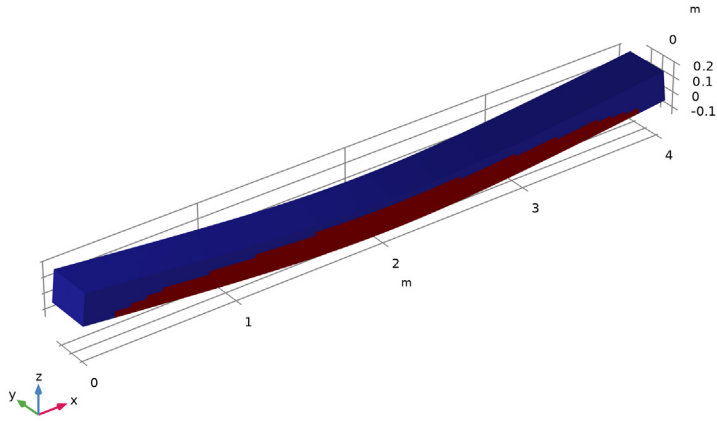
Figure 12: Plastic region in concrete with Ottosen model.
