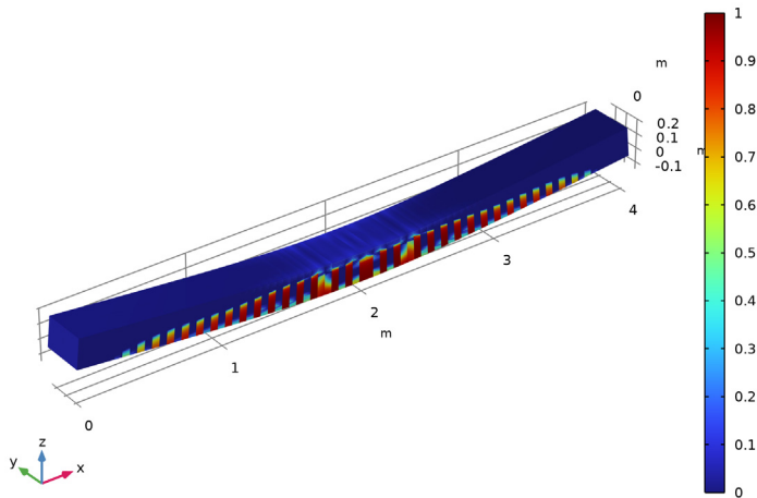
Figure 13: Damaged region in concrete with Mazars damage model.
