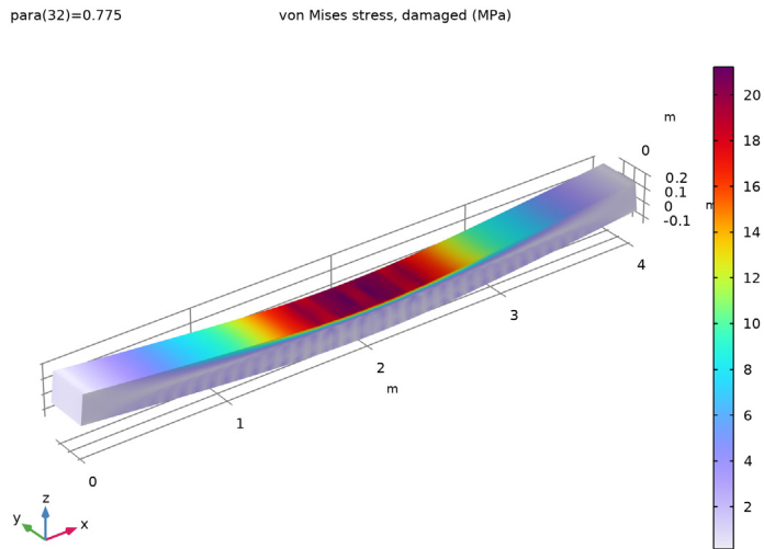
Figure 11: Von Mises stress in reinforced beams when using Mazars damage for the concrete.
