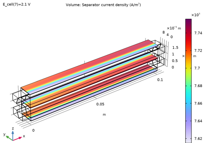
Figure 10: Separator current density.
