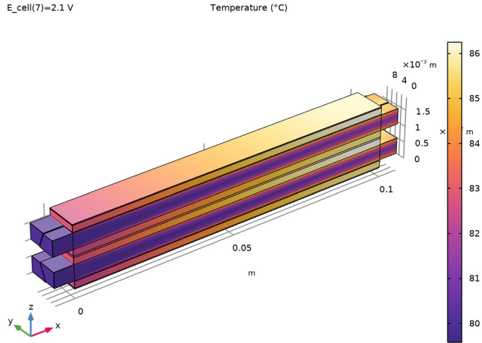
Figure 9: Temperature.
