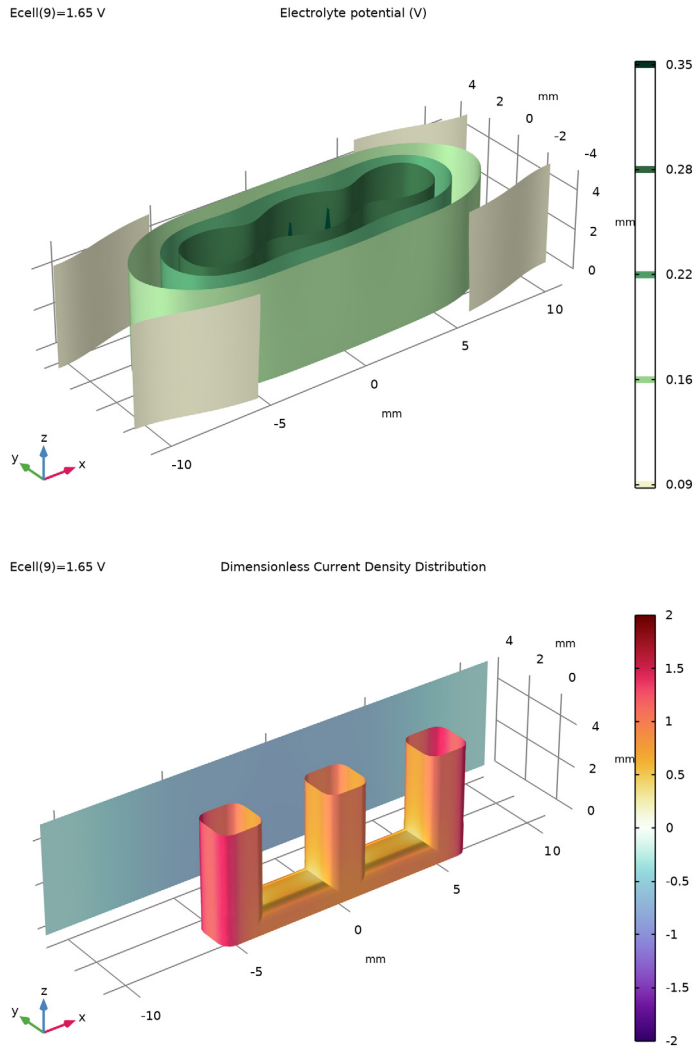
Figure 4: Secondary current distribution, E_{cell} = 1.65 V. Potential distribution in the electrolyte (top) and current density distribution on the anode and posterior cathode (bottom).
