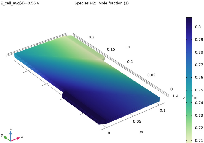
Figure 4: Hydrogen molar fraction.
