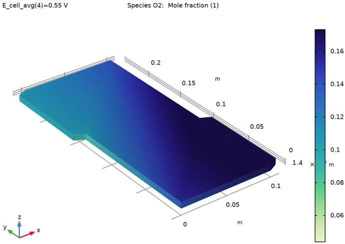
Figure 5: Oxygen molar fraction.
