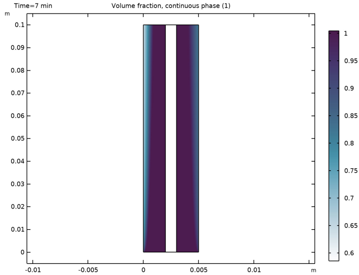
Figure 3: Liquid volume fraction at a cell voltage of 1.9 V.
