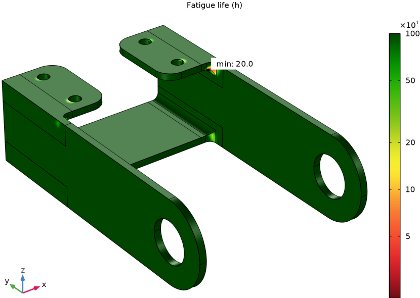
Figure 2: Fatigue life according to Dirlik.
