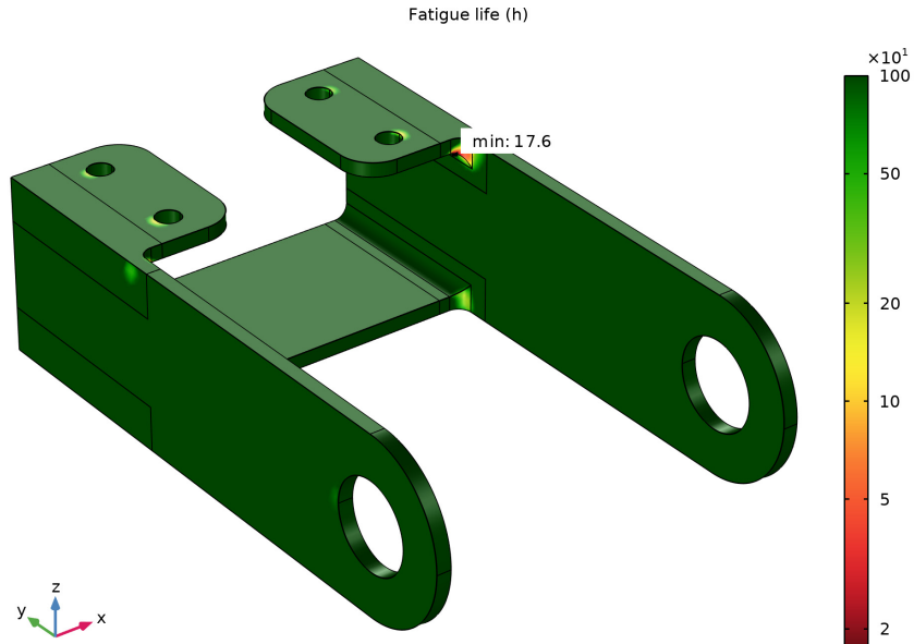
Figure 3: Fatigue life according to Bendat.
