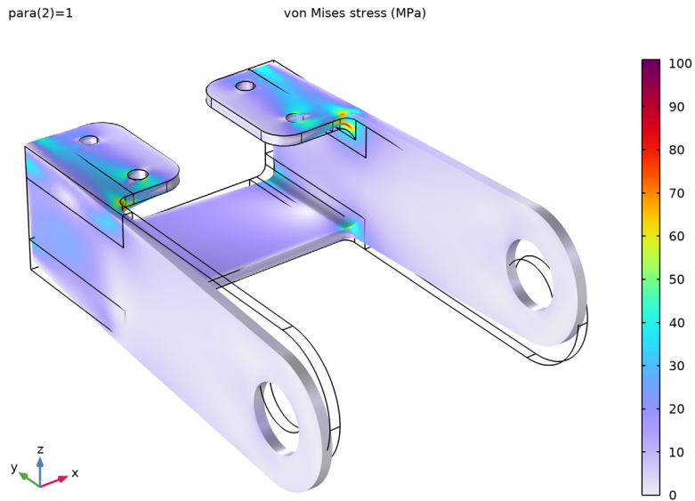
Figure 2: Stress in the bracket at the peak operating load.
