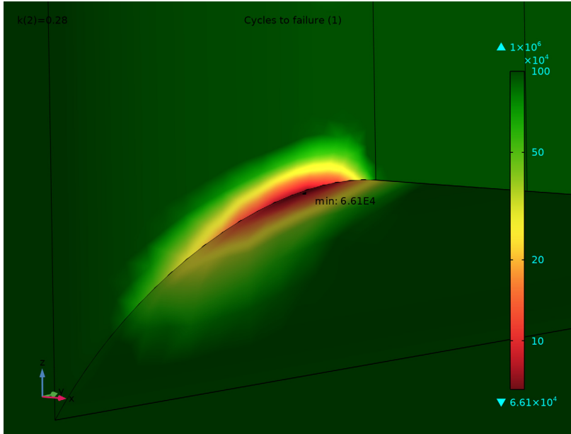
Figure 4: Fatigue lifetime when bracket is submerged in salt water.
