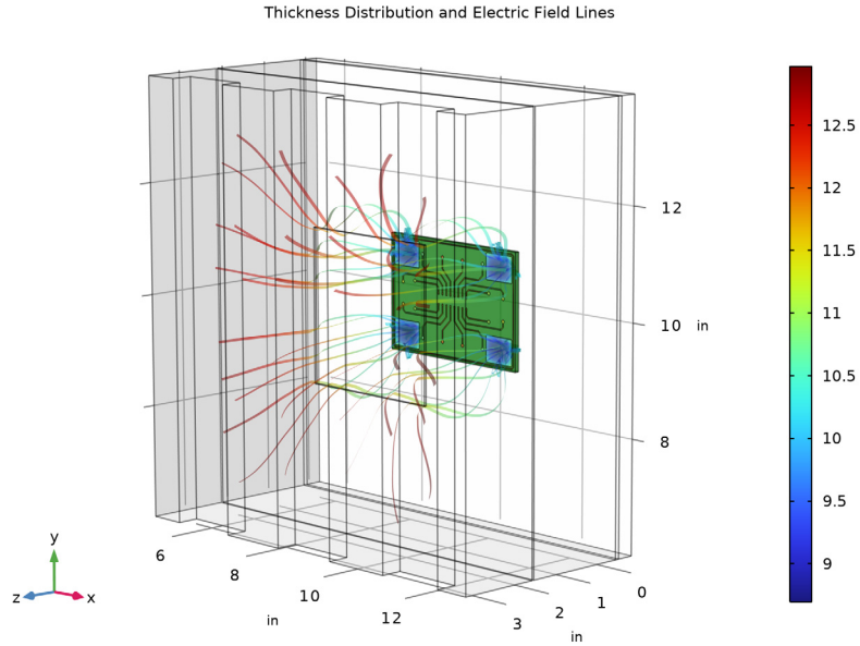
Figure 4: Field lines and thickness on the cathode, including the dummy pattern.
