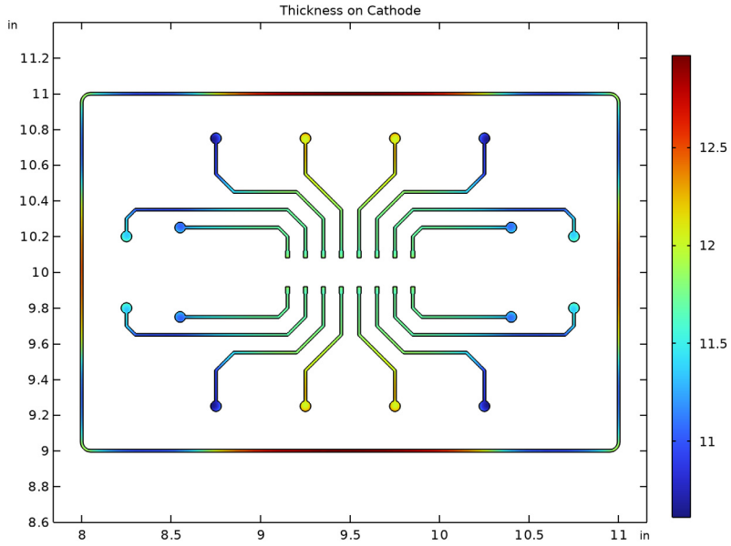
Figure 3: Deposition thickness of the PCB pattern for a target thickness of 10\ \mu\text{m} .
