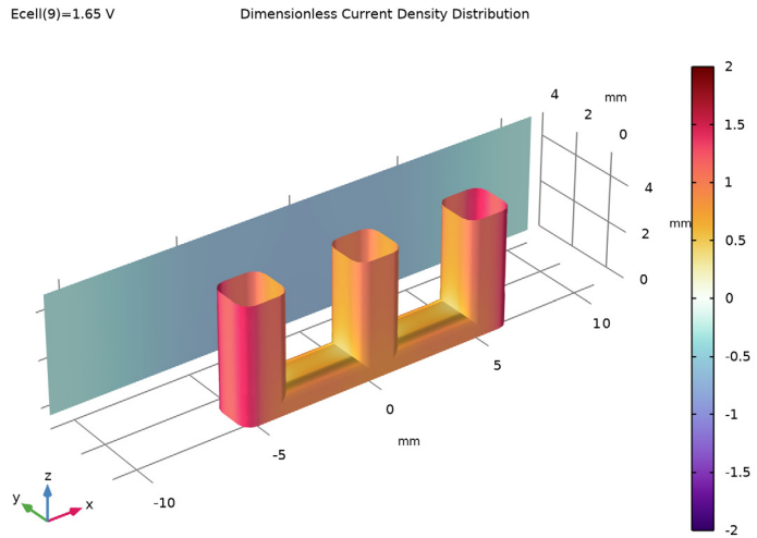
Figure 4: Secondary current distribution, E_{cell} = 1.65 V. Potential distribution in the electrolyte (top) and current density distribution on the anode and posterior cathode (bottom).
