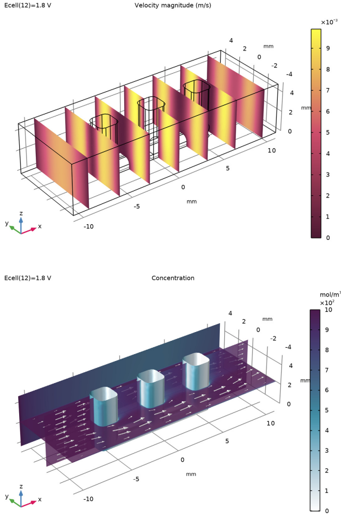
Figure 5: Flow field (top: slice plot, bottom: arrows) and concentration profile (bottom: slices and anode and posterior cathode surfaces) at 1.8 V.
