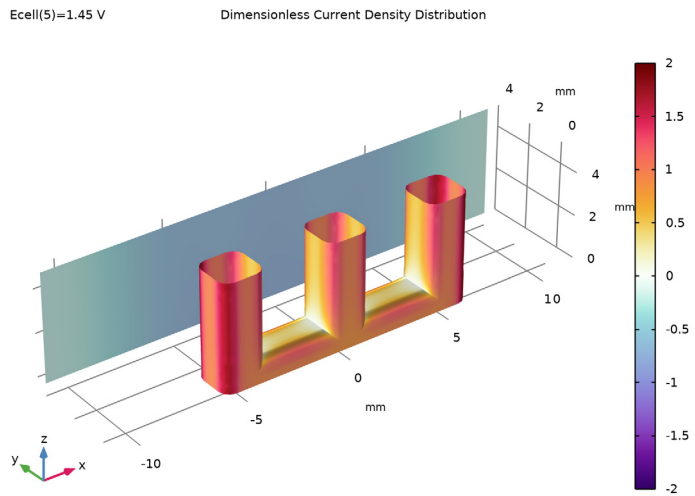
Figure 3: Primary current distribution, E_{cell} = 1.45 V. Potential distribution in the electrolyte (top) and current density distribution on the anode and posterior cathode (bottom).
