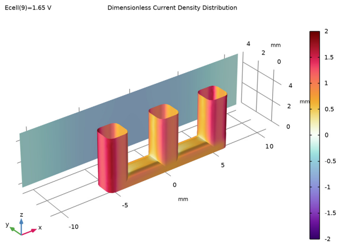
Figure 6: Tertiary current distribution, E_{cell} = 1.65 V. Potential distribution in the electrolyte (top) and current density distribution on the anode and posterior cathode (bottom).
