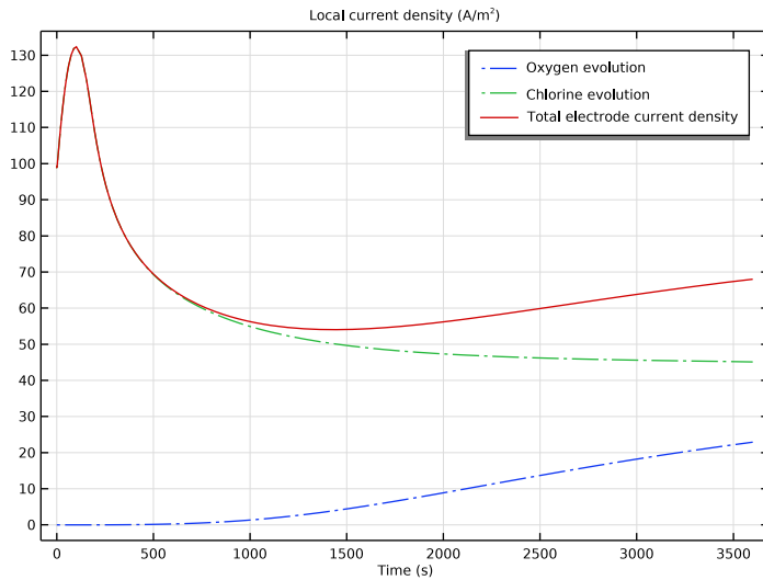
Figure 5: Total current density and current density for the competing reactions on the anode surface. Oxygen evolution is the lowest graph.
