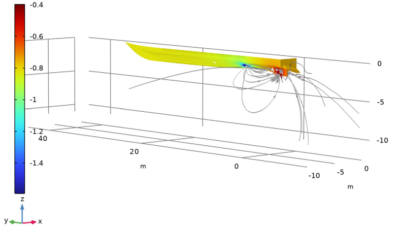
Figure 7: A surface plot of the hull potential for the case of an uncoated propeller.
