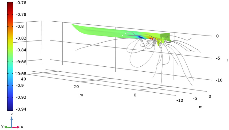
Figure 5: A surface plot of the hull potential for the case with a coated propeller.
