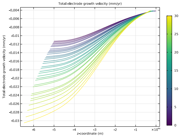
Figure 3: Electrode dissolution rate along the iron electrode surface at various times.
