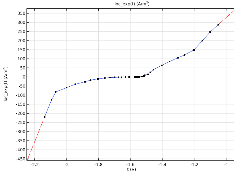
Figure 2: Polarization data for Mg alloy.
