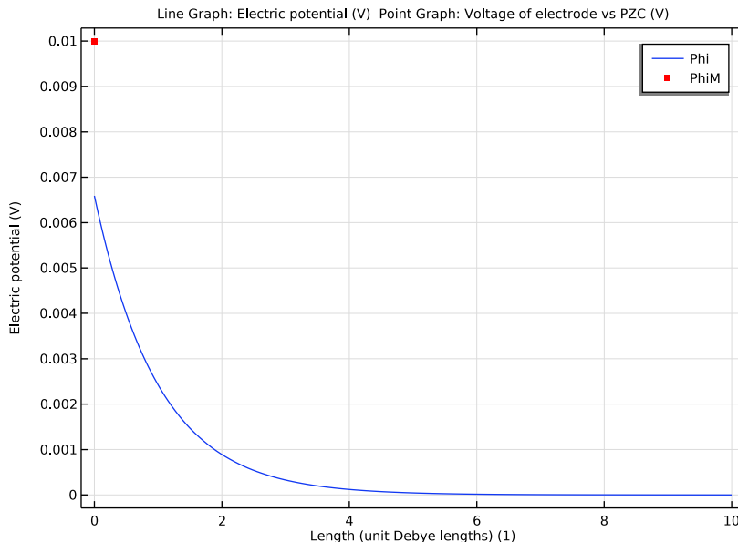
Figure 1: Electrolyte potential profile (blue line) and 10 mV applied electrode potential versus bulk solution (red dot).
