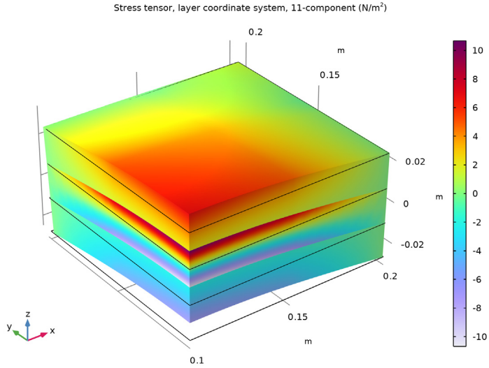
Figure 7: The stress in the fiber direction computed using the ESL theory.
