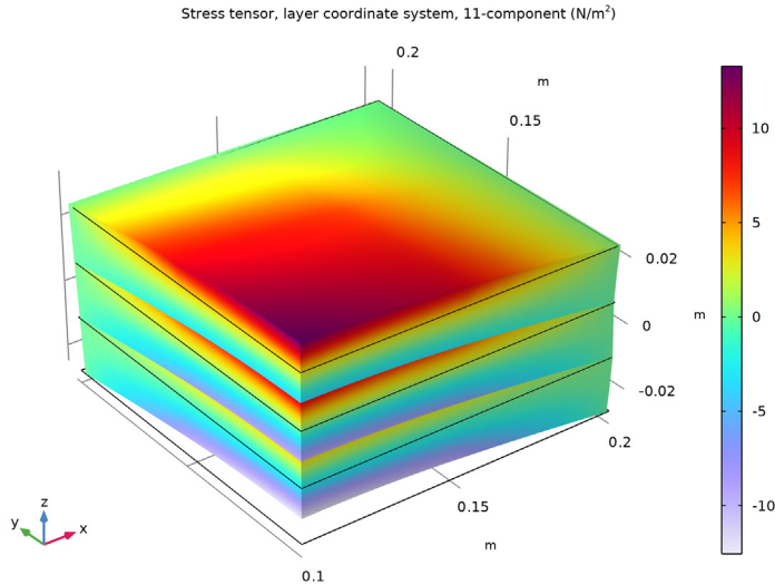
Figure 6: The stress in the fiber direction computed using the layerwise theory.
