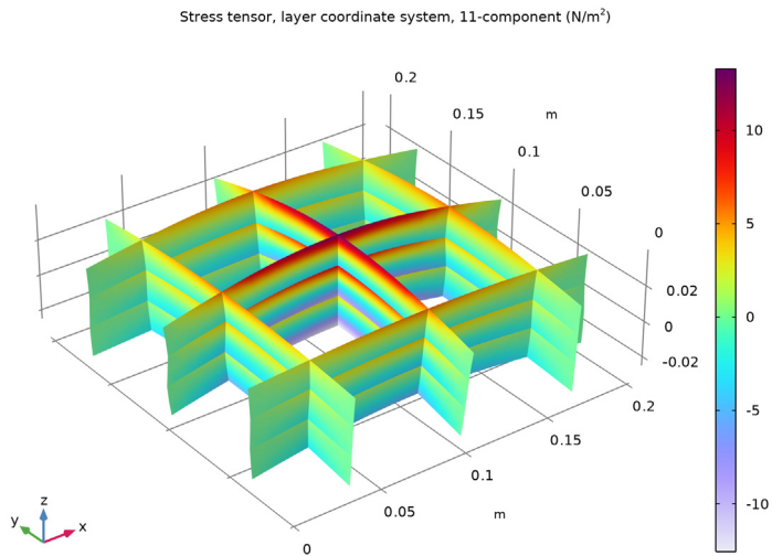
Figure 8: The stress in the fiber direction in the full laminate computed using the layerwise theory.
