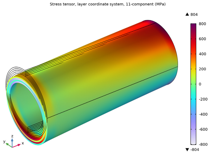
Figure 6: The stress in the fiber direction in the composite laminate.
