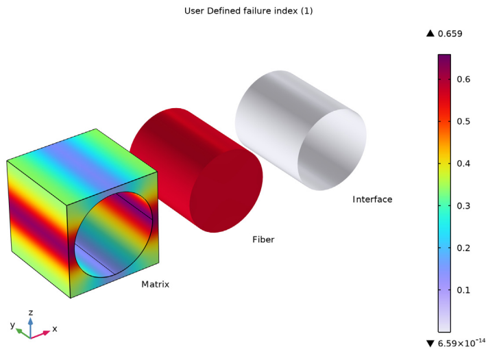
Figure 12: User defined failure indexes in the constituents at a particular material location of the composite cylinder.
