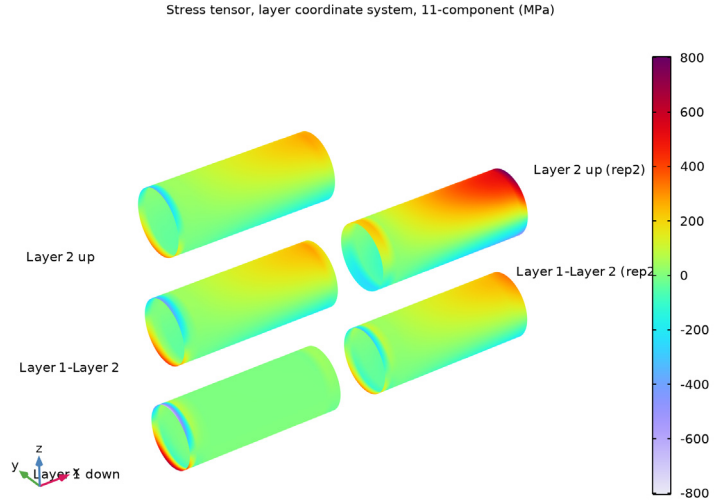
Figure 7: The stress in the fiber direction in the five interfaces of the composite laminate.
