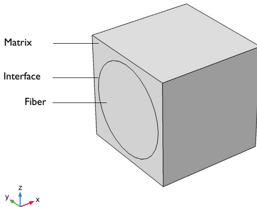
Figure 1: Geometry of the unit cell with a carbon fiber, a thin interface and an epoxy matrix.
