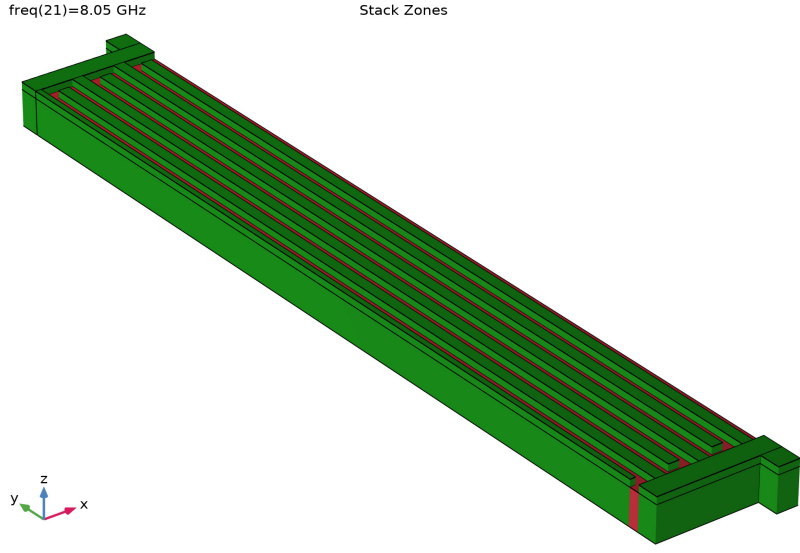
Figure 3: Zones with different layers in the layered shell geometry. The red zone has only aluminum nitride, the green zone has aluminum nitride and platinum layers.
