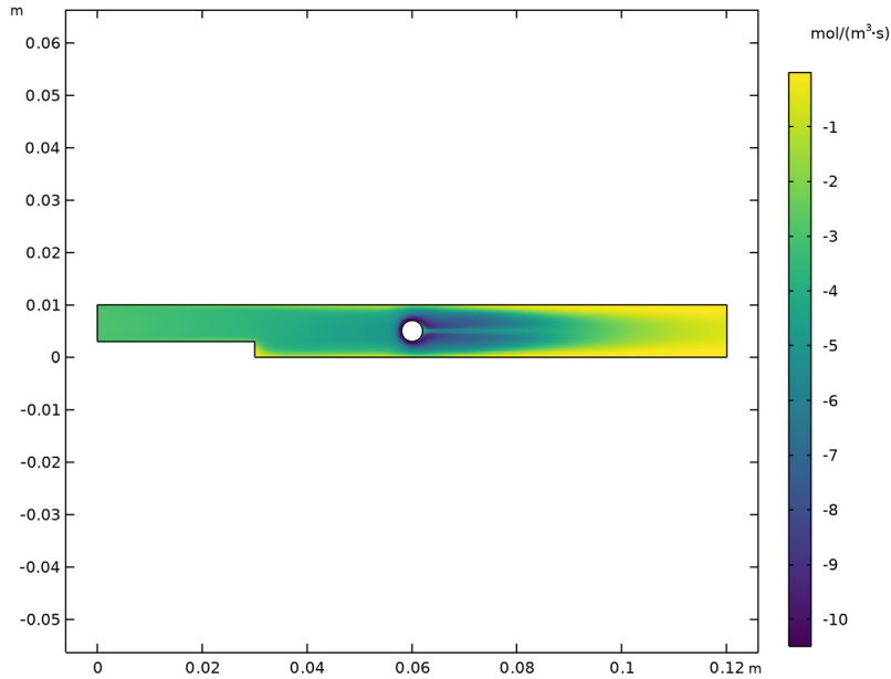
Figure 7: Decomposition rate of compound A. Significant decomposition occurs in the first half of the reactor.
