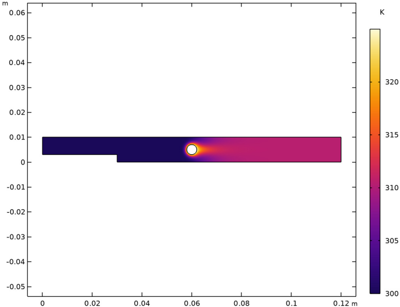
Figure 4: A water solution enters the reactor at 300 K and is heated by a cylinder kept at 325 K.
