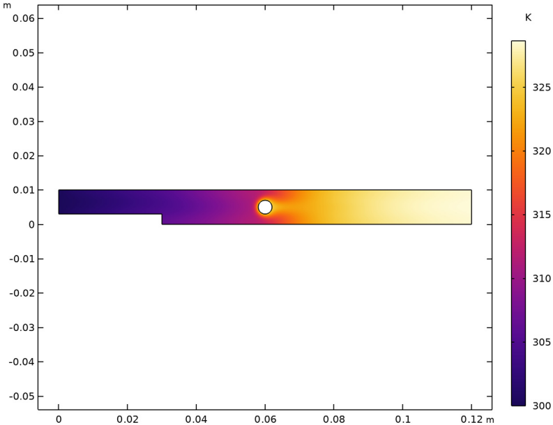
Figure 6: Reactor temperature (K) when the heat of reaction is taken into account.
