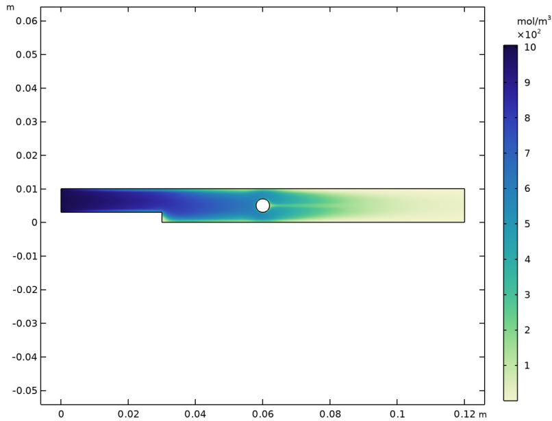
Figure 5: Concentration of the heat sensitive chemical (A) ( \text{mol/m}^3 ) as function of position in the reactor.
