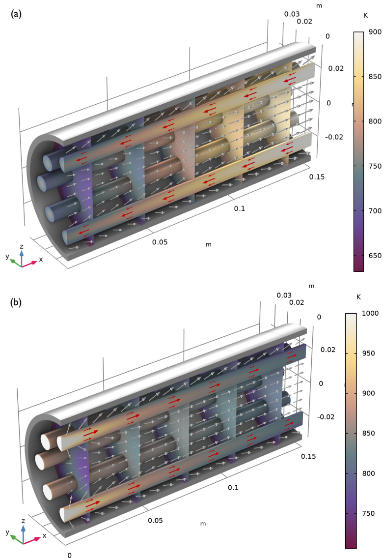
Figure 8: Temperature distributions in the reformer system, including the reformer bed and insulating wall (slices), and heating tubes (surface). Arrows indicate total heat flux on part of the symmetry surface for the bed and heating tubes. (a) Countercurrent setup, (b) Cocurrent 1000 K setup.
