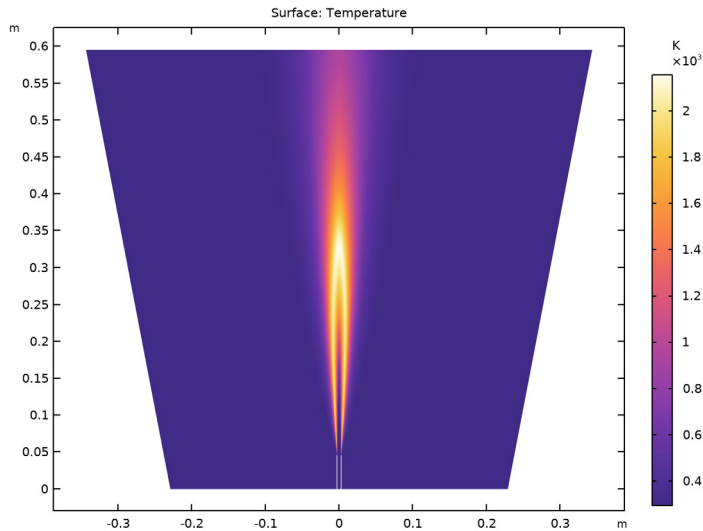
Figure 4: Temperature in the jet.
