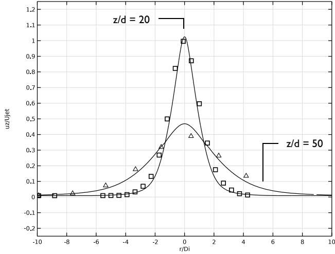
Figure 7: Axial velocity at two different positions downstream of the pipe exit, scaled by the inlet velocity. The radial distance is scaled by the inner diameter of the pipe. Model results are plotted using lines, while experimental results are indicated using symbols.
