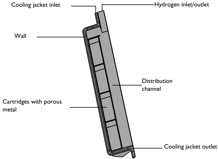
Figure 2: Model geometry including the domain and boundary labels.
