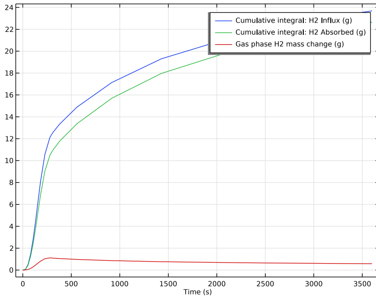
Figure 4: Hydrogen mass profile over time in the gas as well as in the solid phase.
