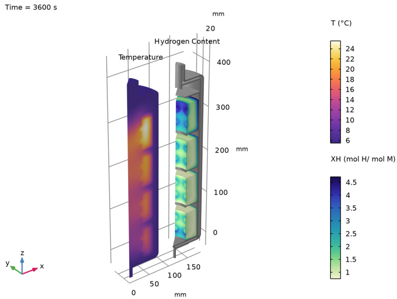
Figure 3: Temperature and hydrogen content XH at 3600 s.
