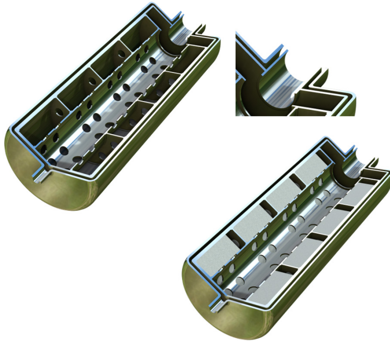
Figure 1: Tank reactor design used in this example.
