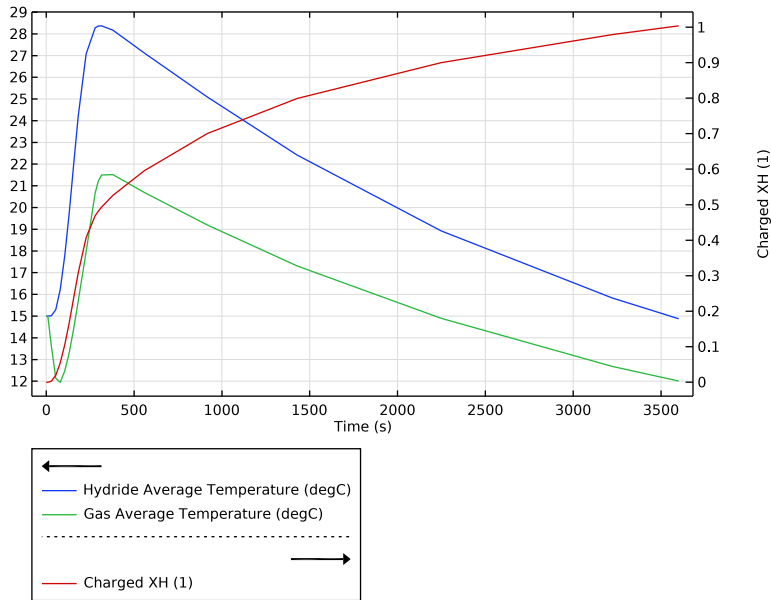
Figure 5: Gas phase temperature, bed temperature, and charged hydrogen content XH over time.
