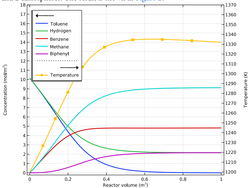
Figure 2: Concentration ( \text{mol}/\text{m}^3 ) and temperature (K) as function of reactor volume ( \text{m}^3 ) for a tubular reactor design.
