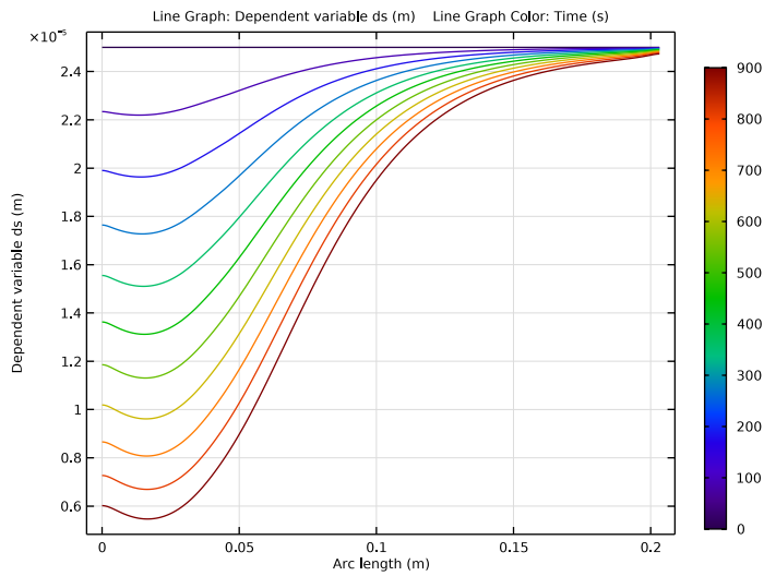
Figure 9: Soot-layer thickness along a channel located at the filter periphery (top) and at the filter centerline (bottom).
