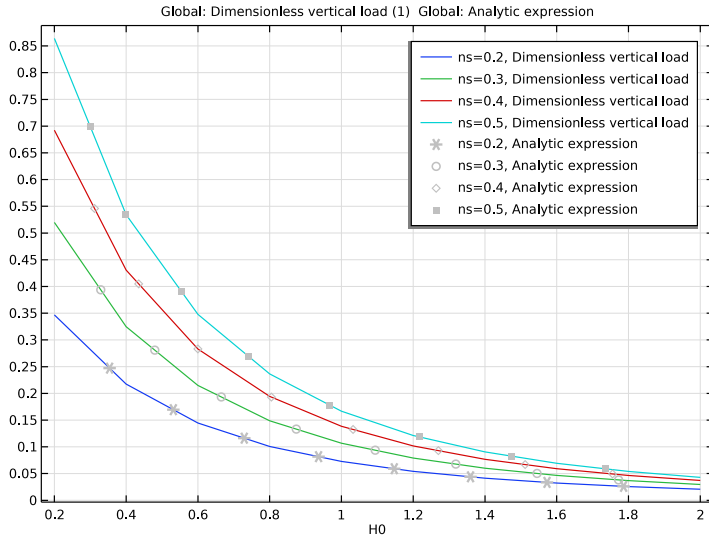
Figure 5: Nondimensional vertical load vs film thickness ratio, H_0 = h_0/s_h . The computed results are shown as the continuous curve and the theoretical result as gray symbols. Different values of the step location n_s = L_s/L are shown.
