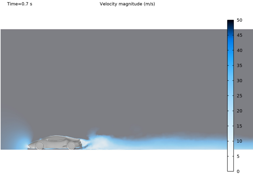
Figure 5: Velocity magnitude in m/s from the LES solution at t = 0.7 s.
