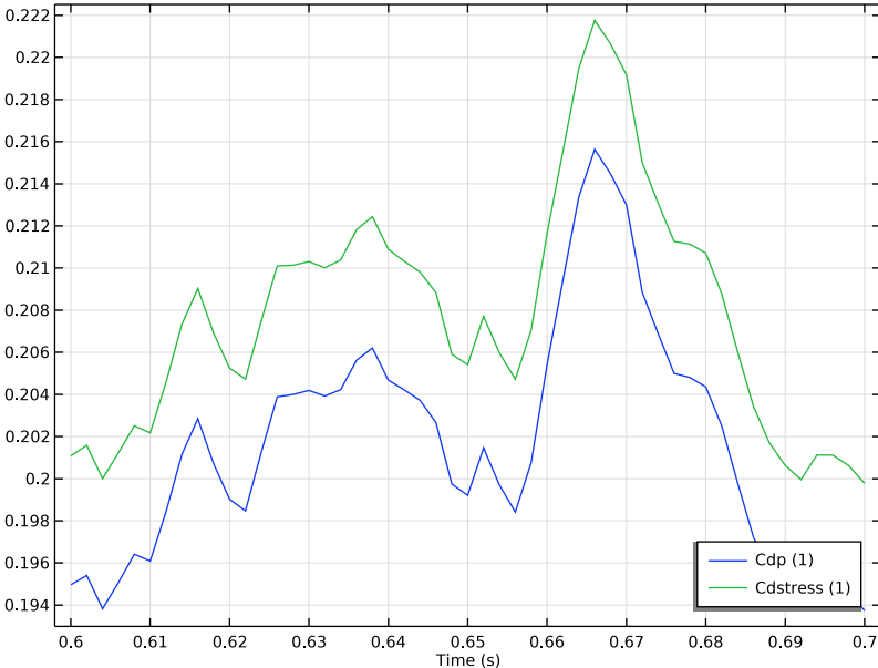
Figure 6: Drag coefficients based on form drag (blue) and total drag (green) from the LES solution between t = 0.6 s and t = 0.7 s.
