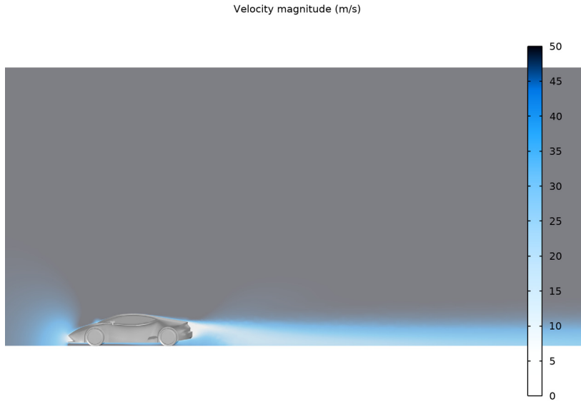
Figure 4: Velocity magnitude in m/s from the RANS k-\epsilon solution.
