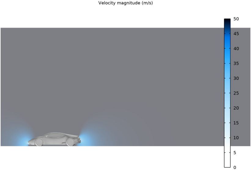
Figure 3: Velocity magnitude in m/s from the potential-flow solution.
