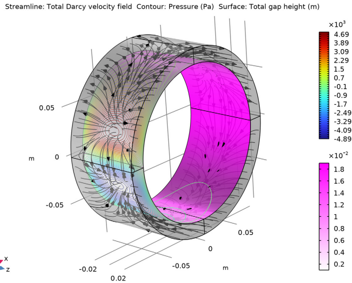
Figure 8: Streamlines showing the flow of lubricant in the porous bush of a self-lubricating journal bearing. Also shown are the contours of pressure and the variation of thickness of the thin film of fluid in the gap between the bush and the journal.
