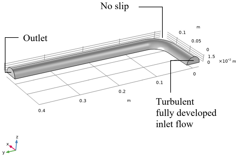
Figure 1: Pipe elbow geometry.
