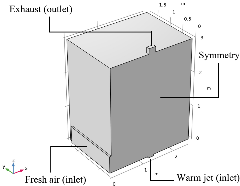
Figure 1: The modeling domain is reduced to half the chamber size due to symmetry.
