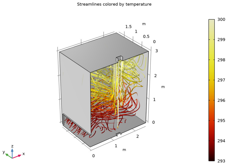
Figure 2: Streamlines colored by the temperature illustrating the velocity field.
