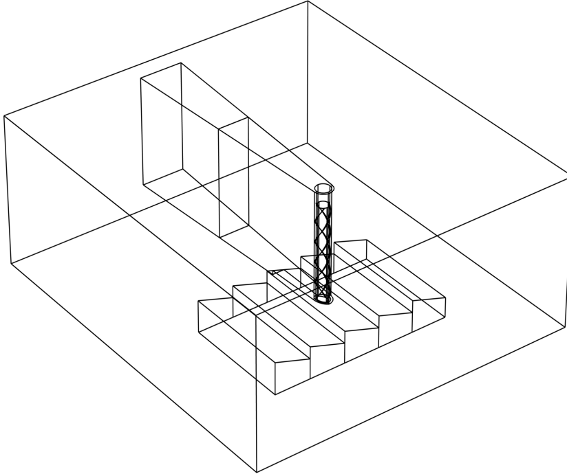
Figure 1: Geometry of the computational domain with mesh domains included downstream of the chimney.
