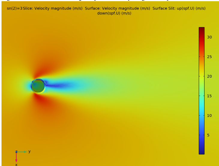
Figure 5: Horizontal slice plot of the velocity magnitude for the model with strakes.
