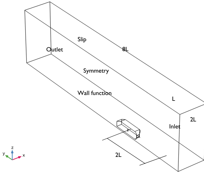
Figure 2: The size of the computational domain is reduced by mirror symmetry.
