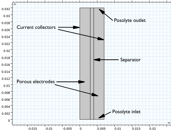
Figure 2: Model Geometry.
