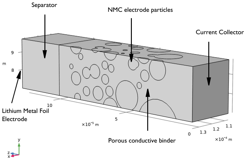
Figure 1: Model geometry.
