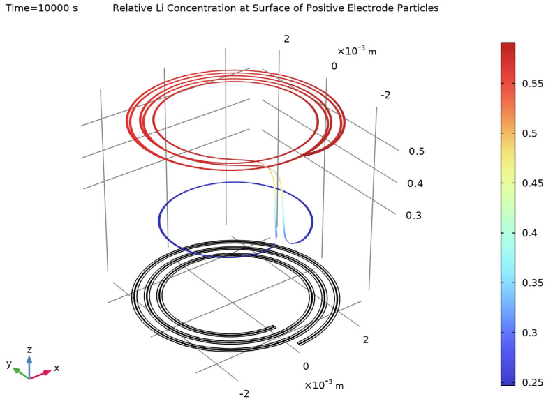
Figure 13: Relative lithium concentration at the surface of the positive electrode particles at t = 10,000 s for the relaxation simulation.
