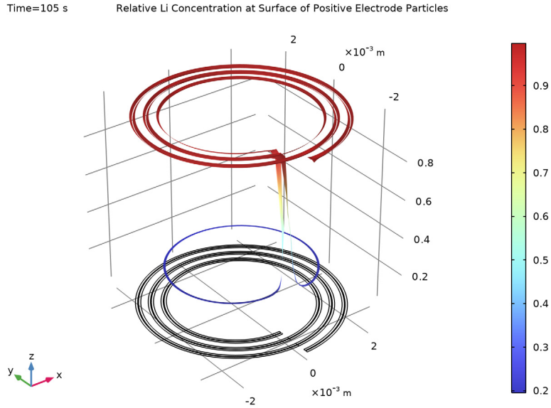
Figure 8: Relative lithium concentration at the surface of the positive electrode particles at t = 105 s for the 10C discharge.
