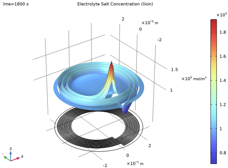
Figure 5: Electrolyte salt concentration at t = 1800 \text{ s} for the 1C discharge.
