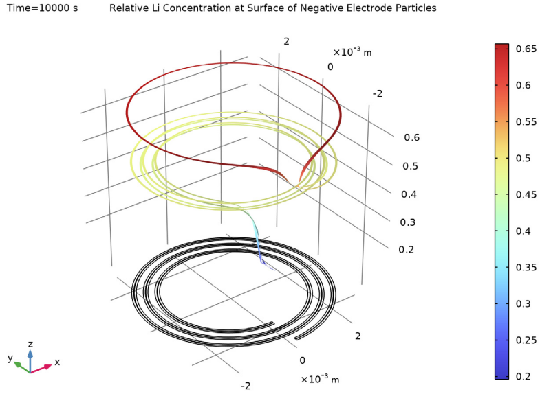
Figure 12: Relative lithium concentration at the surface of the negative electrode particles at t = 10,000 s for the relaxation simulation.
