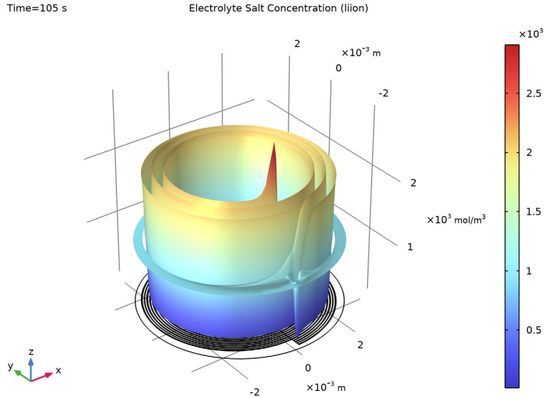
Figure 9: Electrolyte salt concentration at t = 105 s for the 10C discharge.
