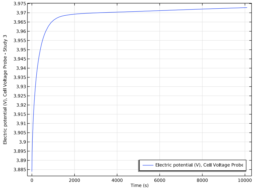
Figure 10: Cell potential versus time during the relaxation simulation.
