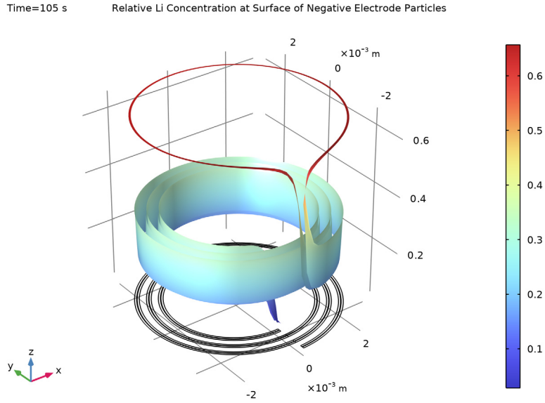
Figure 7: Relative lithium concentration at the surface of the negative electrode particles at t = 105 s for the 10C discharge.
