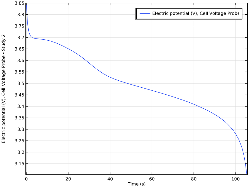
Figure 6: Cell potential versus time during the 10C discharge.
