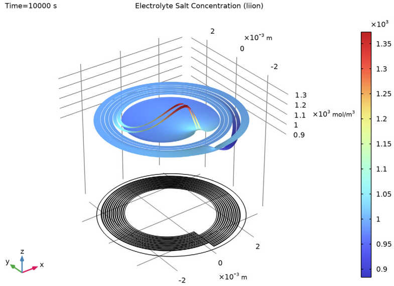
Figure 11: Electrolyte salt concentration at t = 10,000 s for the relaxation simulation.
