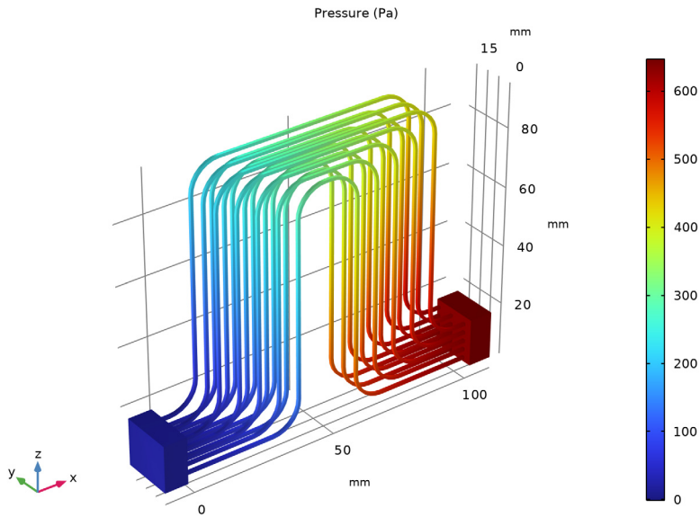
Figure 3: Pressure in the flow compartment.
