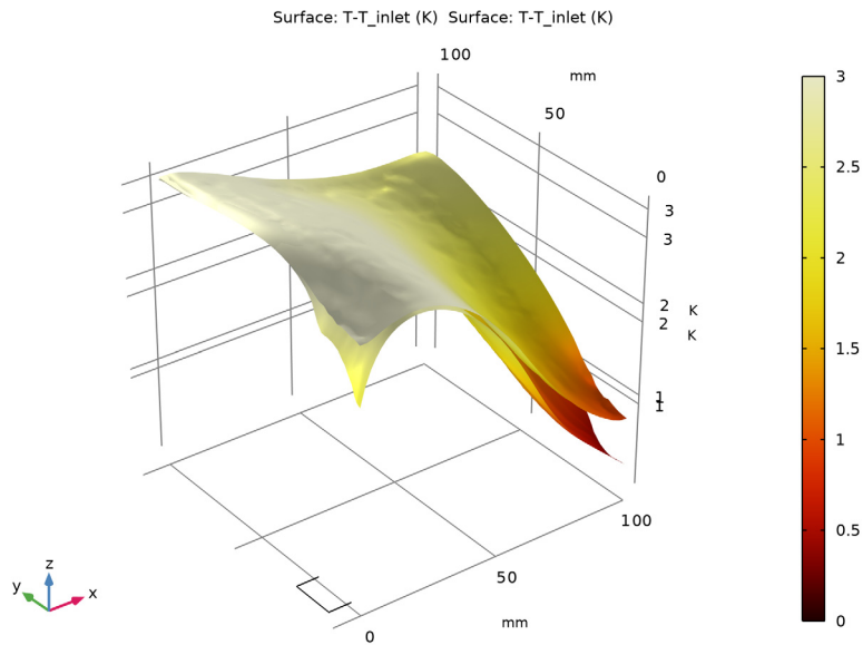
Figure 7: Temperature increase (in relation to the inlet temperature) of the second battery at the surface facing the cooling fin ( y = 4 mm) and the surface facing the third battery ( y = 6 mm).
