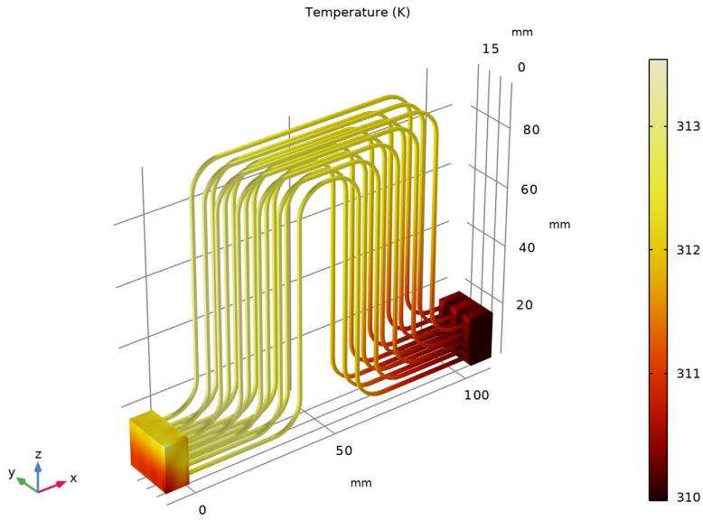
Figure 6: Temperature of the cooling liquid.
