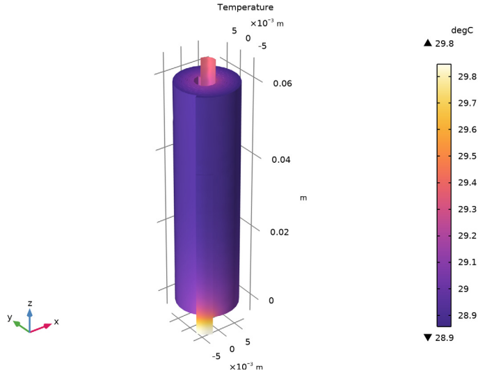
Figure 5: Temperature distribution.
