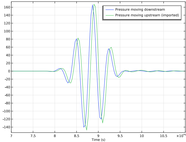
Figure 8: The average acoustic pressure on the receiver for the signal moving downstream (modeled in this tutorial) and the signal moving upstream (data imported).
