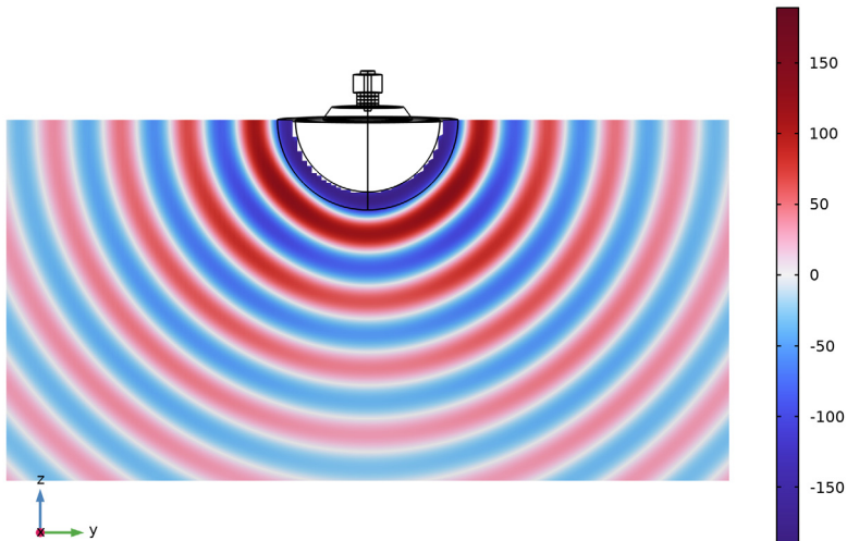
Slice Plot of Exterior Pressure Field
