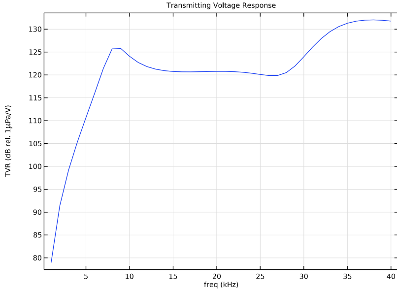
Figure 13: Transmitting Voltage Response (TVR) as a function of frequency obtained at an on-axis distance of 1 m ahead of the head mass and computed relative to 1 \mu Pa/V.
