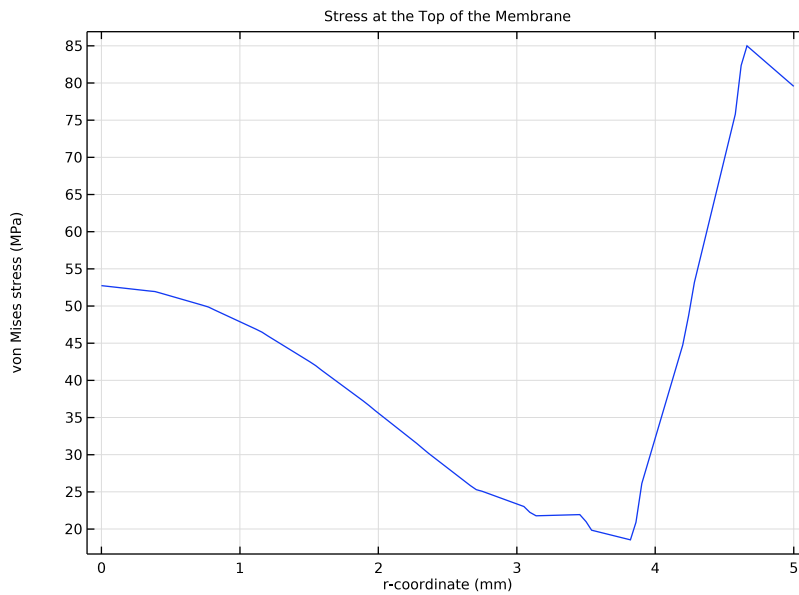
Figure 5: von Mises Stress along the air-solid interface.
