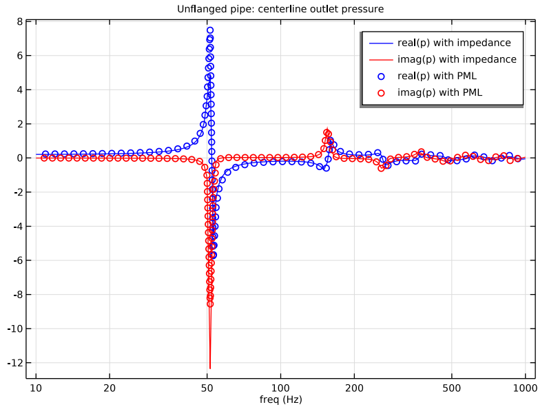
Figure 7: Pressure p at the centerline of the pipe outlet for the unflanged pipe.
