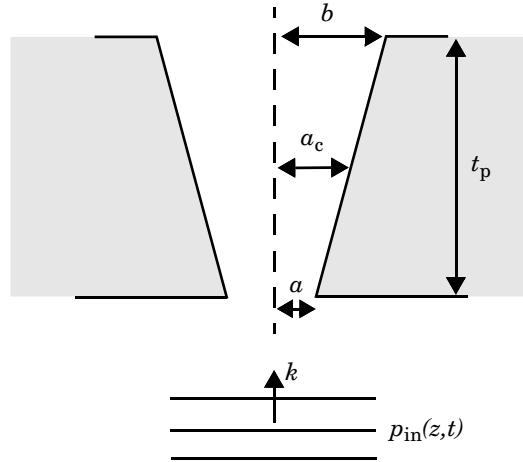
Figure 1: Schematic representation of the tapered orifice in the microperforated plate.
