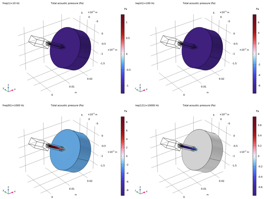
Figure 11: Pressure distribution in the earmold tubing and coupler volume for 10 Hz, 100 Hz, 1 kHz, and 10 kHz.
