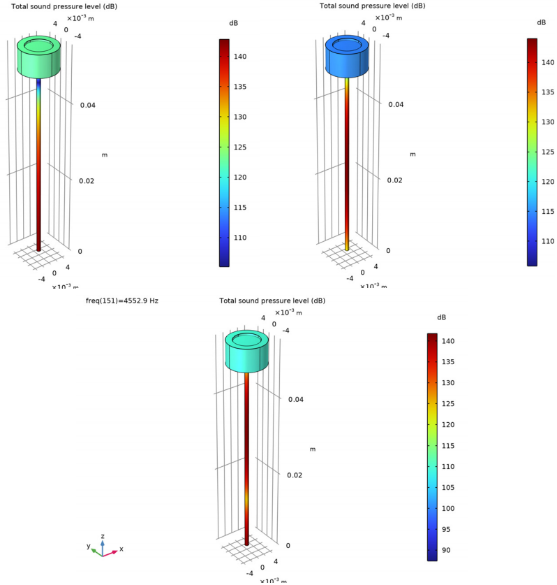
Figure 6: Sound pressure level at frequencies close to f = 1200 , 3200 , and 4600 Hz.
