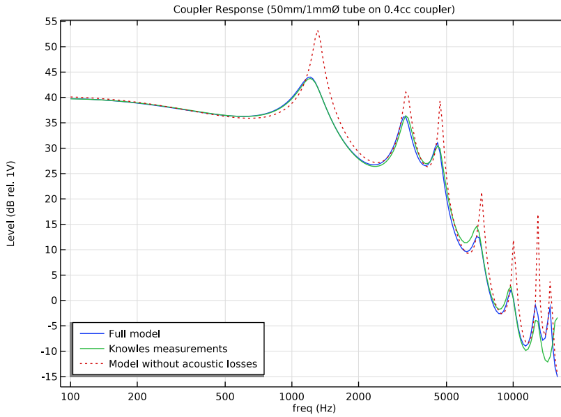
Figure 3: The microphone response comparing the model including the thermal and viscous losses via the narrow region acoustics feature (blue curve), the model without acoustic losses (red dotted curve), and measurements (green curve). Measurement data provided by Knowles, IL, USA.
